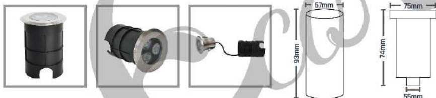
Diagram On Left - Plastic Housing Diagram On Right - 304 Stainless Steel
